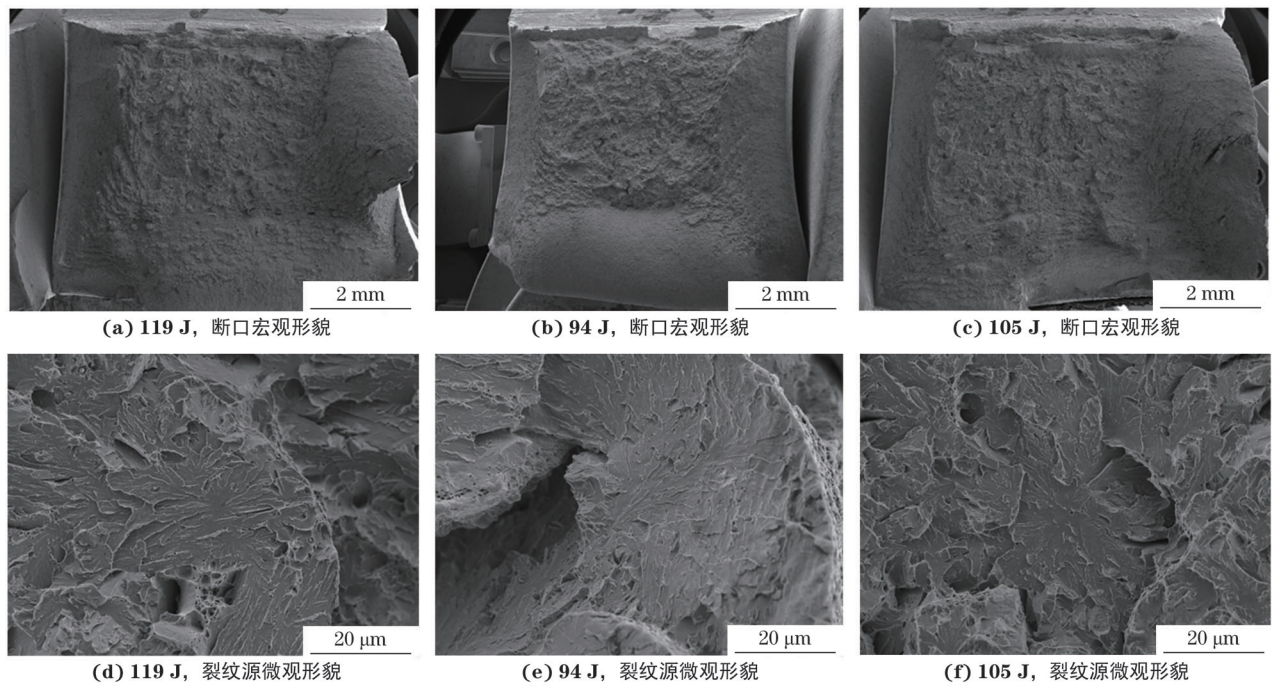
图 2 55\text{ }^{\circ}\text{C}\cdot\text{h}^{-1} 焊后热处理冷却速率下不同冲击吸收能量的焊缝金属断口宏观形貌与裂纹源微观形貌 (道间温度 250\text{ }^{\circ}\text{C} ) Fig. 2 Fracture macromorphology (a-c) and crack initiation source micromorphology (d-f) of weld metal with different impact absorbed energies at post-weld heat treatment cooling rate of 55\text{ }^{\circ}\text{C}\cdot\text{h}^{-1} (interpass temperature of 250\text{ }^{\circ}\text{C} )
