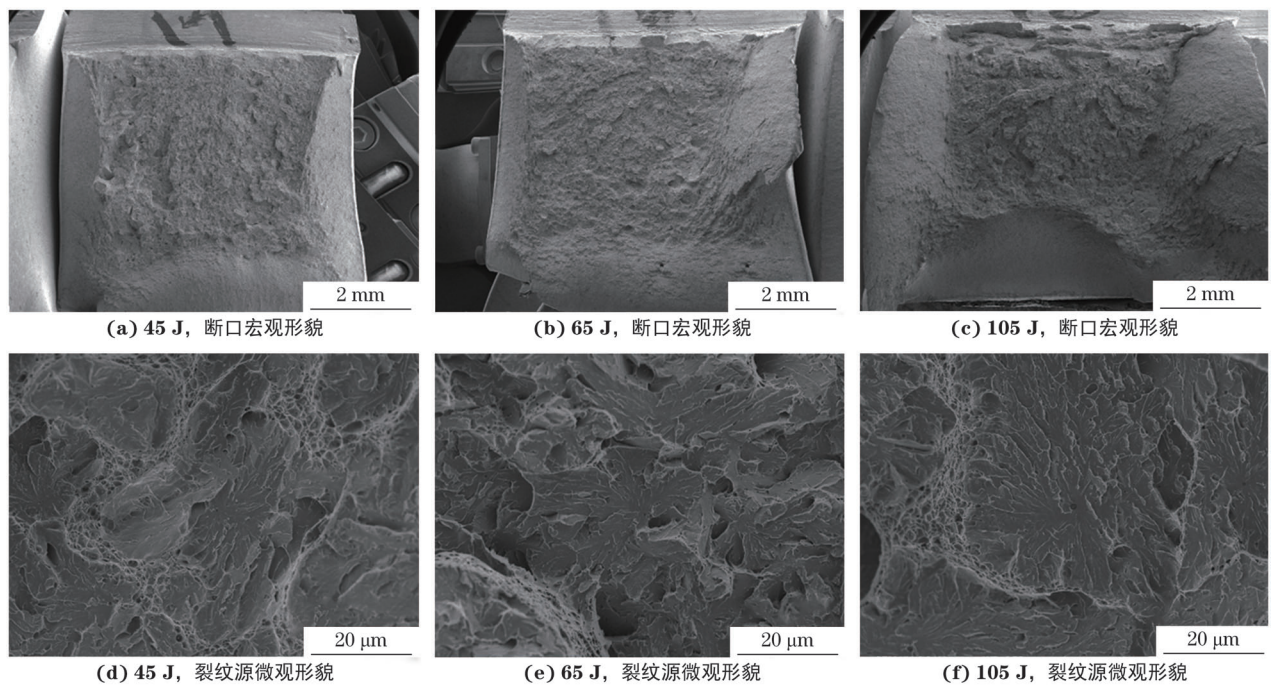
图 3 约 20\text{ }^{\circ}\text{C}\cdot\text{h}^{-1} 焊后热处理冷却速率下不同冲击吸收能量的焊缝金属断口宏观形貌与裂纹源微观形貌 (道间温度 250\text{ }^{\circ}\text{C} ) Fig. 3 Fracture macromorphology (a-c) and crack initiation source micromorphology (d-f) of weld metal with different impact absorbed energies at post-weld heat treatment cooling rate of about 20\text{ }^{\circ}\text{C}\cdot\text{h}^{-1} (interpass temperature of 250\text{ }^{\circ}\text{C} )
